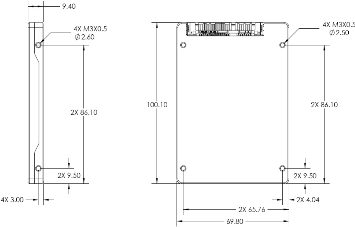
Figure 2: Kingston SSDNow V+ series Mechanical Drawing
